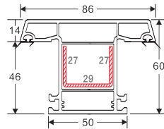
CASEMENT DOOR MULLION Weight: 1.130 Code: 3D 60-47 (G) 6 Pieces/Bag
