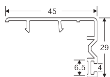
INTERLOCK Weight: 0.227 Code: 3D 60-15 (A) 30 Pieces/Bag
