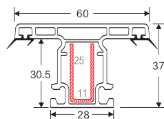
SASH MULLION Weight: 0.636 Code: 3D 60-17 (G) 6 Pieces/Bag
