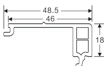
BLINDS SHUTTER Weight: 0.255 Code: 3D 60-33 (A) 20 Pieces/Bag
