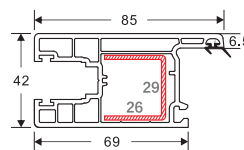
MEGA SASH Weight: 1.250 Code: 3D 60-14 (G) 4 Pieces/Bag
