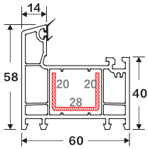
CASEMENT FRAME Weight : 1.050 Code: 3D 60-1 (G) 6 Pieces/Bag
