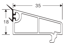
CASEMENT SINGLE GLAZING BEAD Weight: 0.317 Code: 3D 60-5 (G) 20 Pieces/Bag
