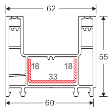
TWO TRACK SLIDING FRAME Weight: 1.098 Code: 3D 60-11 (A) 6 Pieces/Bag
