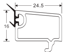
SLIDING SINGLE GLAZING BEAD Weight: 0.270 Code: 3D 60-16 (G) 20 Pieces/Bag
