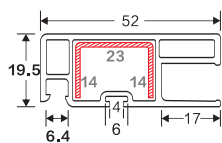
SLIDING MESH SASH Weight: 0.492 Code: 3D 92-2 (A) 15 Pieces/Bag
