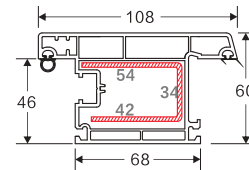
CASEMENT OUTWARD SASH Weight: 1.650 Code: 3D 60-6 (G) 4 Pieces/Bag
