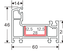
SMALL CASEMENT FRAME Weight: 0.850 Code: 3D 60-2 (A) 6 Pieces/Bag
