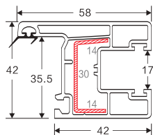
SMALL SASH Weight: 0.840 Code: 3D 60-12 (G) 8 Pieces/Bag
