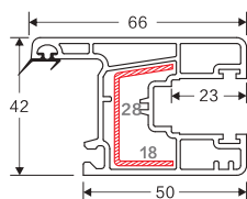
BIG SASH Weight: 1.042 Code: 3D 60-13 (G) 8 Pieces/Bag
