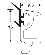
SLIDING SINGLE GLAZING BEAD Weight: 0.270 Code: 3D 60-16 (G) 20 Pieces/Bag
