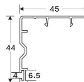
BLINDS SHUTTER Weight: 0.255 Code: 3D 60-33 (A) 20 Pieces/Bag
