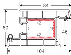
CASEMENT INWARD SASH Weight: 1.650 Code: 3D 60-10 (G) 4 Pieces/Bag
