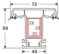
MULLION Weight: 1.130 Code: 3D 60-3 (O) 6 Pieces/Bag
