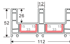
THREE TRACK FRAME Weight: 1.700 Code: 3D 60-112 (A) 4 Pieces/Bag
