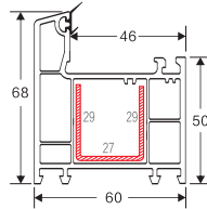
CASEMENT DOOR FRAME Weight: 1.277 Code: 3D 60-9 (G) 6 Pieces/Bag
