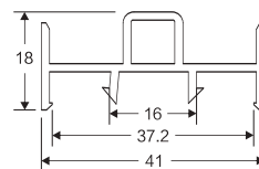
INLINE ADOPTOR Weight: 0.332 Code: 3D 60-7 (A) 20 Pieces/Bag
