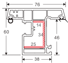
CASEMENT WINDOW SASH Weight: 1.210 Code: 3D 60-2 (A) 6 Pieces/Bag
