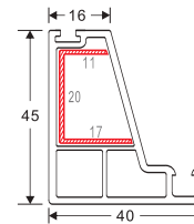
CASEMENT DOOR MULLION Weight: 1.130 Code: 3D 60-47 (G) 6 Pieces/Bag
